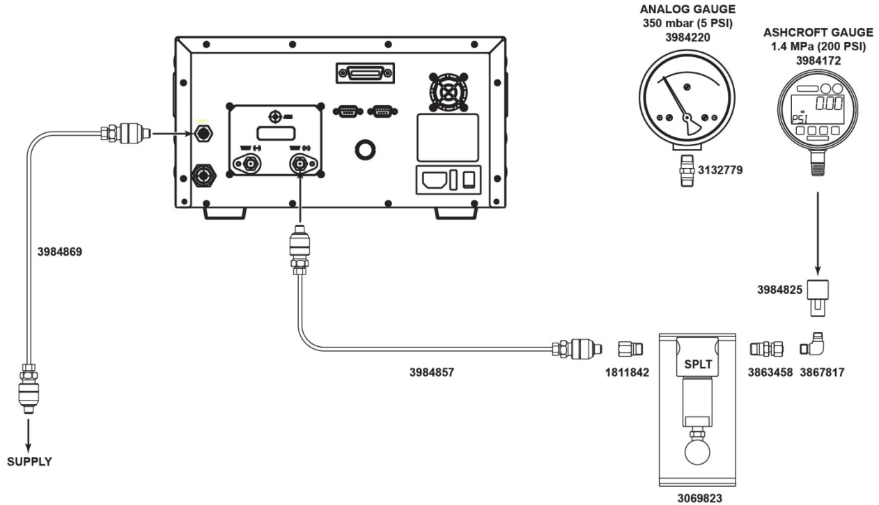
Figure 2: 1.4 MPa PPC4E Demo Kit Assembly
